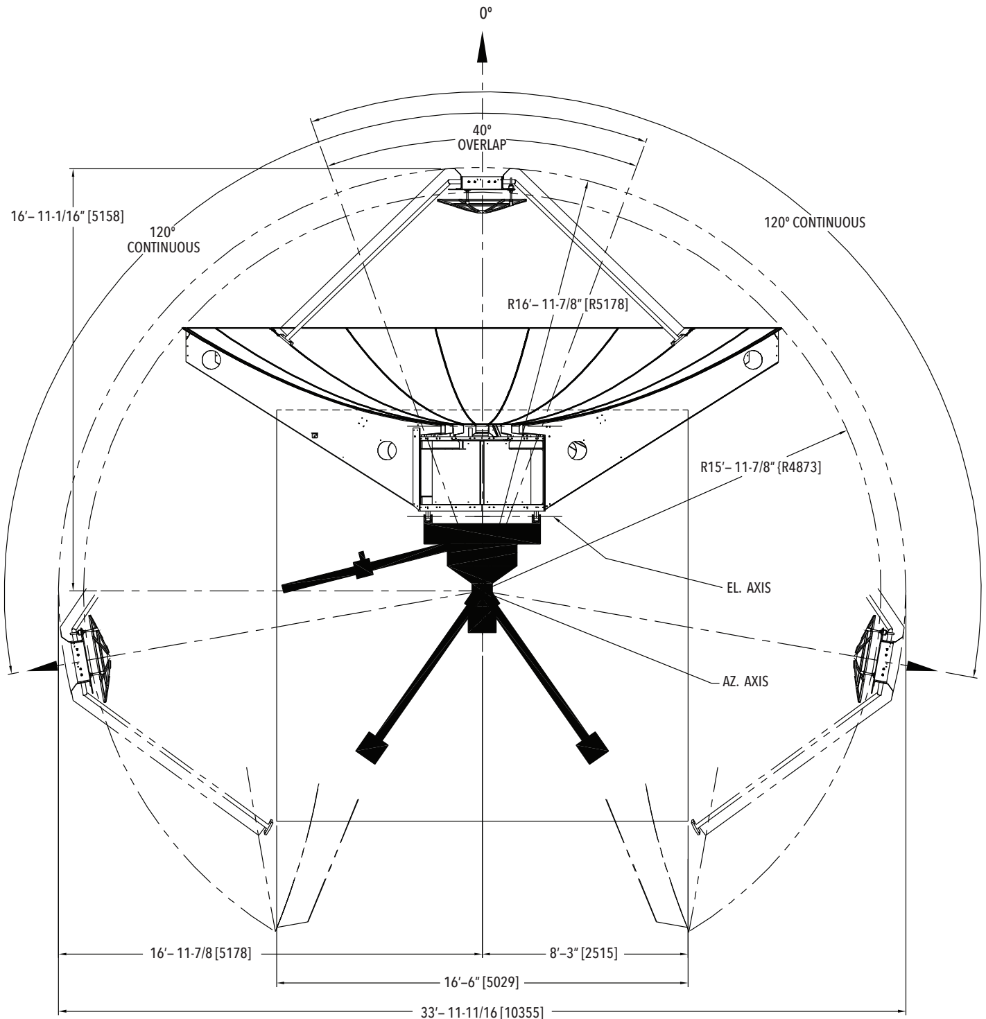
PLAN VIEW
